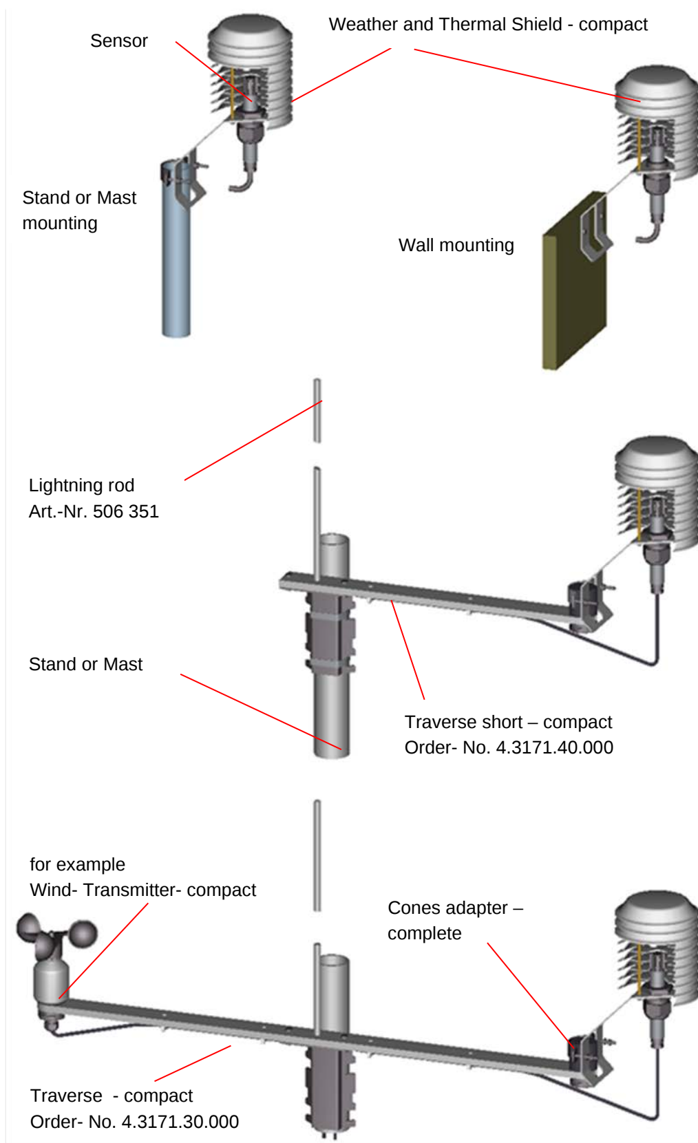
Figure 1: Mounting possibilities
